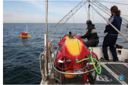
Fig. 4 – AEGIR two-body AUV from Cartagena University
