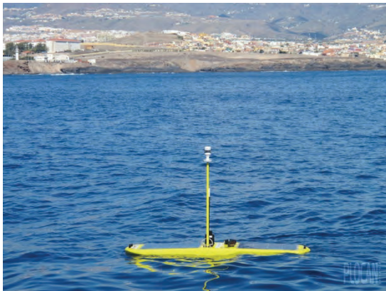
Fig. 5 A new concept of glider: Waveglider technology.
