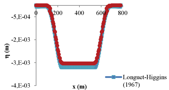
Figure 4 – Mean surface elevation. Comparison between Longuet-Higgins(1967) solution and TELEMAC3D/TOMAWAC coupling.
