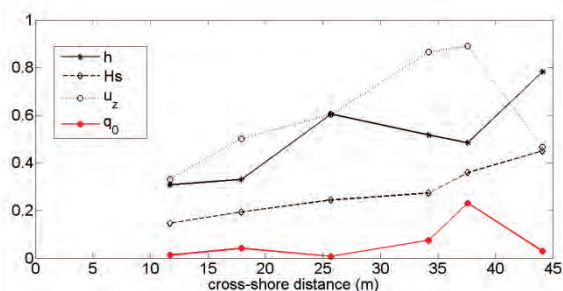
Fig. 5. Cross-shore distribution of water depth, h (m); significant wave height, H_s (m); current velocity in longshore direction at 0.23 m from the bottom, u_z ( \text{ms}^{-1} ) and sedimentary flux at the bottom, q_0 ( \text{kgm}^{-2}\text{s}^{-1} ).
